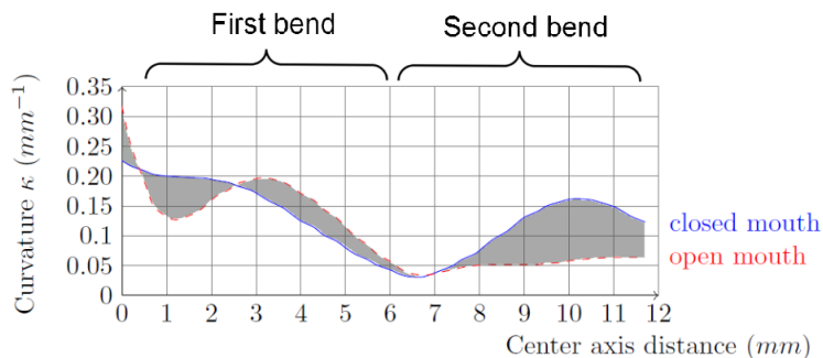
FIG. 4. Curvature alignment of the center axes for the two extreme positions. The area between two curves (in gray) is proportional to the available bending energy
