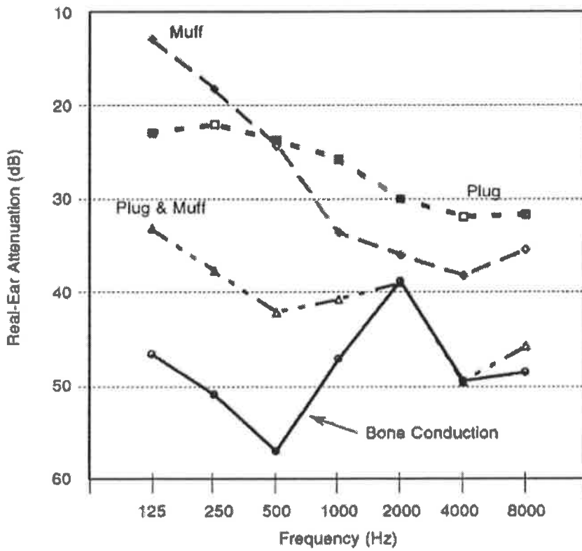
FIG.4 (PRIOR ART)
